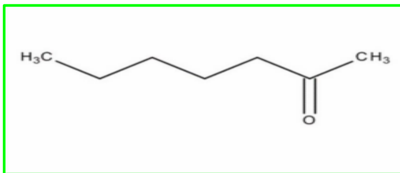
Molecular Structure
