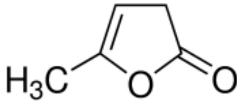
Molecular Structure
